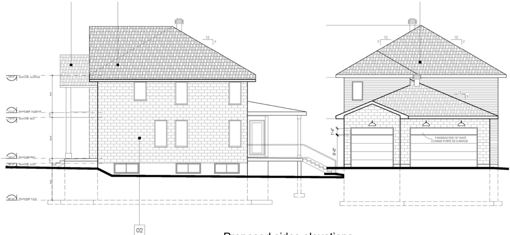
Proposed sides elevations
